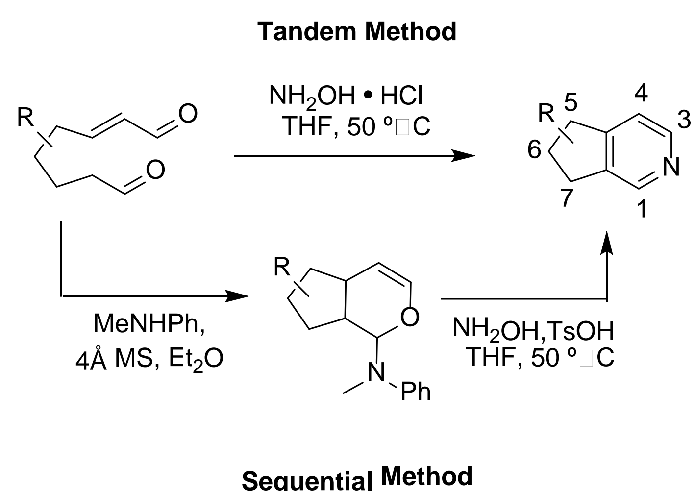
Isolated Yields Of Substituted Cyclopenta[C]Pyridine (6)
