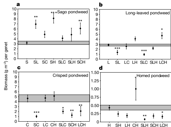
Figure 2 Biomass yield (mean ± s.e.) per genet (shoot biomass per individual planted) of the four submerged macrophyte species (a–d) in monocultures and in mixed cultures. C, crisped pondweed; H, horned pondweed; L, long-leaved pondweed; S, sago pondweed. Biomass per genet standardizes the number of individuals planted in different mixtures (21 individuals in monocultures, 10 individuals per species in bicultures, and 7 individuals per species in tricultures). A species experienced interspecific competition if its biomass per genet was significantly lower ( P < 0.05) in the presence of other macrophyte species than in monoculture. * P < 0.05, ** P < 0.01 and *** P < 0.001, in contrasts after analysis of variance.
