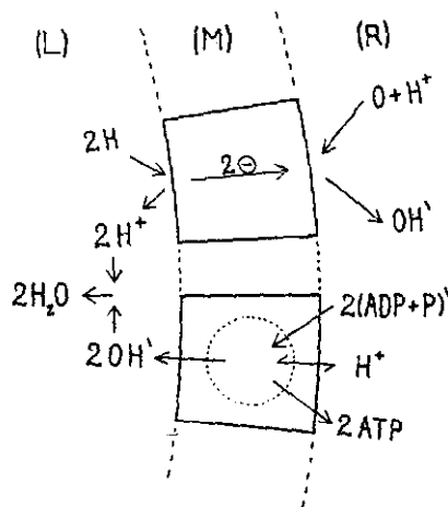
Fig. 2. Electron transport system (above) and reversible 'ATPase' system (below) chemiosmotically coupled in a charge-impermeable membrane (M) enclosing aqueous phase L in
